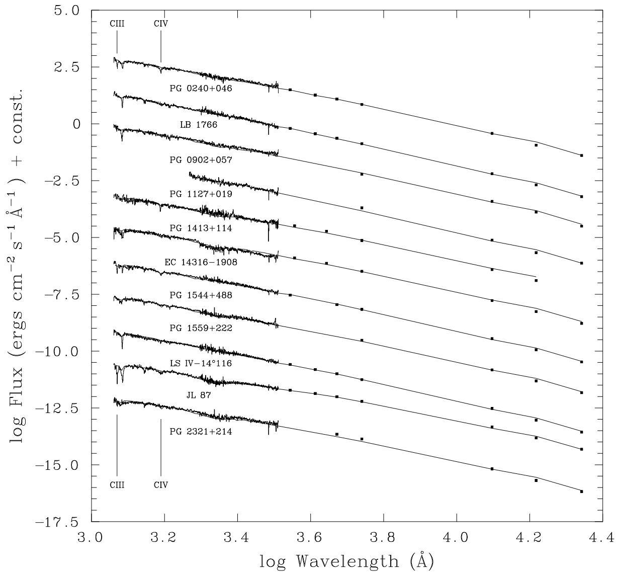
Fig. 1. Flux distribution of He-sdB stars with the model fits.
