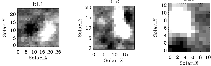
Fig. 1. Partial frame of BBSO magnetograms of the three blinker examples. The images are obtained by averaging over 15 minutes and are scaled from -15 to 15 Gauss. The units in Y and X axes are ‘arcsec’.
