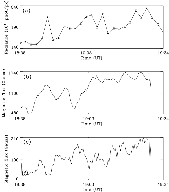
Fig. 9. a) CDS O v 629 Å radiance profile of blinker BL3 obtained by integrating over the blinker area; b) The total magnetic flux from positive polarity fragments above 40 Gauss; c) The total magnetic flux from negative polarity fragments above 25 Gauss.
