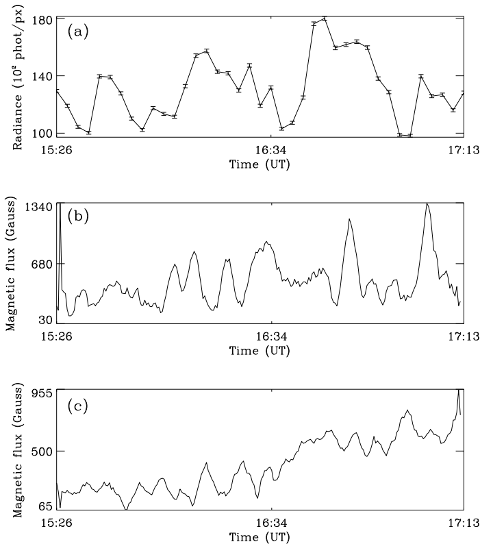
Fig. 7. a) CDS O v 629 Å radiance profile of blinker BL1 obtained integrating over the blinker area; b) The total magnetic flux from positive polarities fragments above 40 Gauss; c) The total magnetic flux from negative polarities fragments above 25 Gauss.
