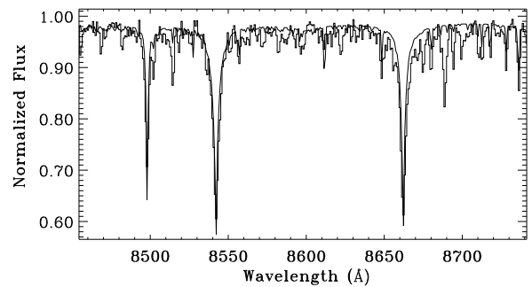
Fig. 3. Normalized red spectrum of the composite PG 2110+127 around the infrared calcium triplet (histogram) together with the best fit model spectrum (poly-line).
