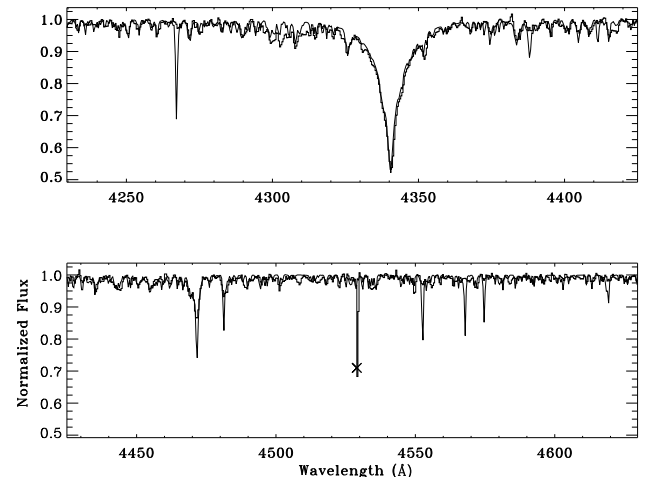
Fig. 4. As in Fig. 1 but for the composite sdB star PG 2148+095.
