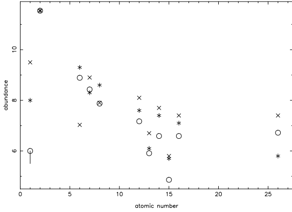
Fig. 5. Chemical abundances of LSS 3184 (circles), V652 Her (crosses), and typical hot EHe (asterisks) vs atomic number. The H abundance for LSS 3184 is an upper limit.
