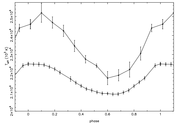
Fig. 4. T_{\text{eff}} vs phase for LSS 3184. The upper curve displays the results from this paper. The lower curve displays results of UV and visible flux fitting in Woolf & Jeffery (2000).
