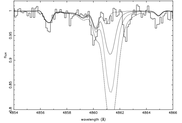
Fig. 6. H\beta region of observed LSS 3184 spectrum and synthetic spectra with H = 4.0, 6.0, 8.0, 8.5, and 9.0 . H = 4.0 and 6.0 are identical.
