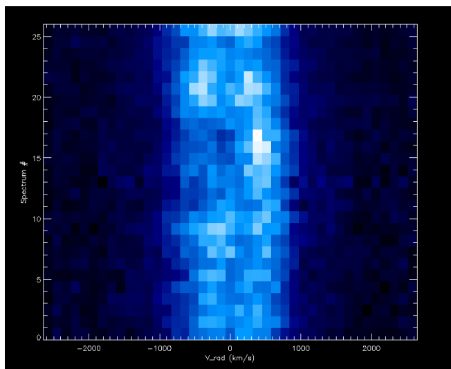
Figure 5. The stacked spectra showing the H \alpha emission line taken on Oct 6 2008 when the source was in a quiescent state. Each spectrum has been normalised so the continuum is unity and time increases vertically.
