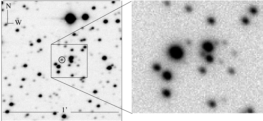
Figure 2. Left hand panel: The white light finding chart for RAT J1953+1859 made using the Wide Field Camera on the INT in June 2005. The circle shows the position of RAT J1953+1859. Right hand panel: The image taken the NOT on Sept 28th 2008 – RAT J1953+1859 was \sim 4 mag brighter than in the INT image.
