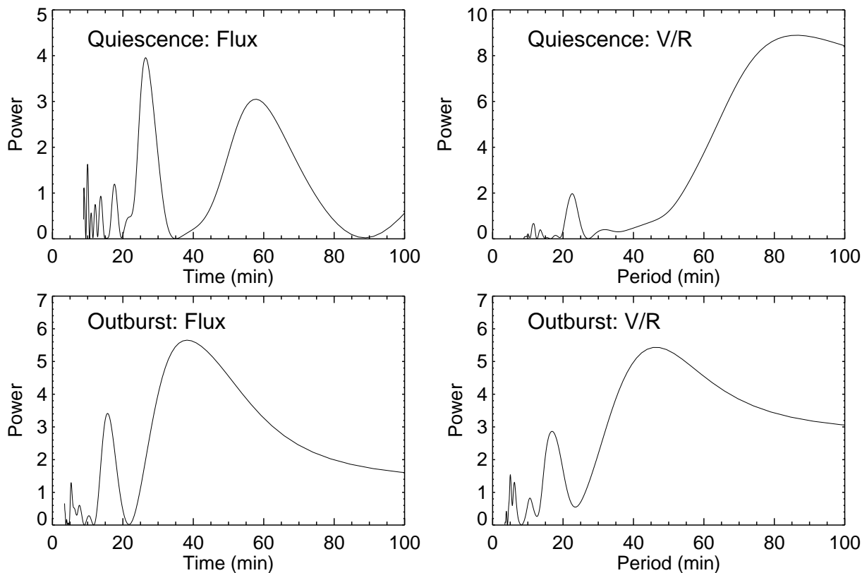
Figure 6. The top panel shows the power spectra of the flux (left hand panel) and the V/R ratio (right hand panel) of the H \alpha line in quiescence. In the lower panel we show the same plots made using data taken in outburst (in Oct 2008).
