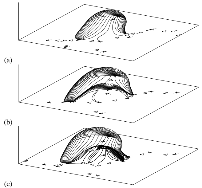
Fig. 4. Three-dimensional fieldline extrapolations showing the important topological separatrix surfaces for each of the three phases of the blinker group. (a) The overlying separatrix dome which contains all the flux from P1 and bounds the entire blinker group region. (b) The appearance of P2 creates a new separatrix dome inside the pre-existing one. (c) The internal dome plays host to a new coronal null point.
