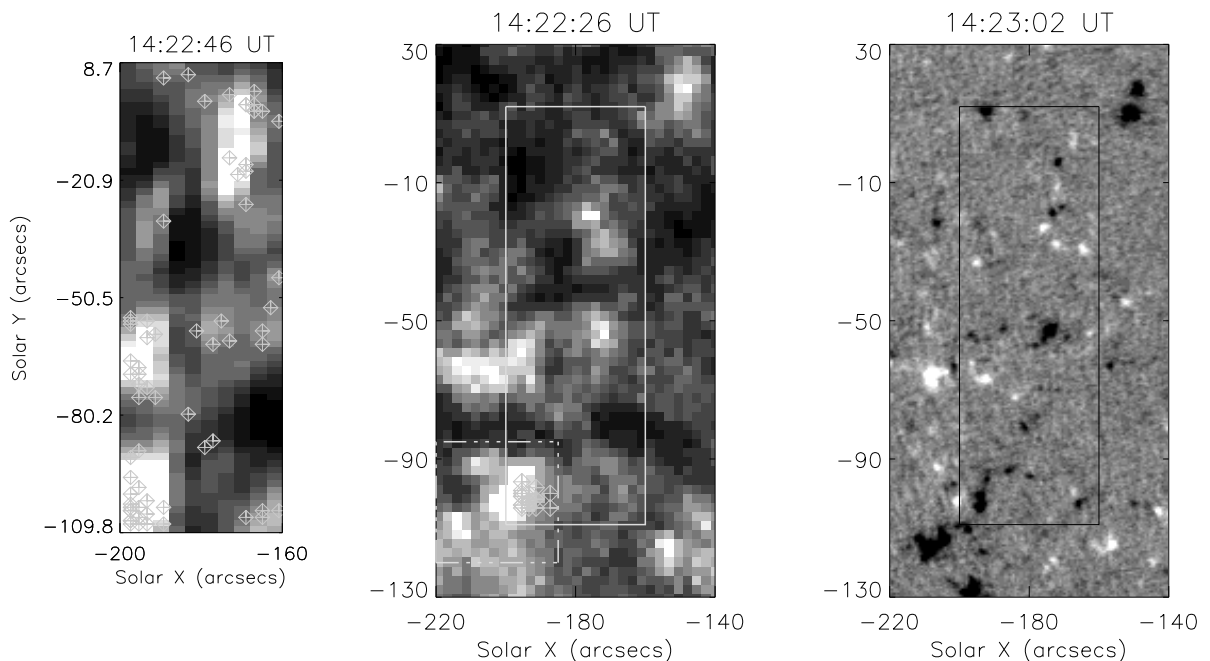
Fig. 1. CDS O v 629 Å raster (left). The diamonds mark the positions of blinkers identified with BLIP. EIT image in the He II 304 Å passband (middle). The solid line box shows the field-of-view of the CDS raster, the dot-dot-dot-dash box shows the field-of-view of the TRACE 1550 Å images presented further in this paper. The blinkers shown with diamonds in the lower left-hand corner of the CDS and TRACE 1550 Å fields-of-view were further analysed and modelled. MDI magnetogram (right) with a black solid box marking the position of the CDS FOV.
