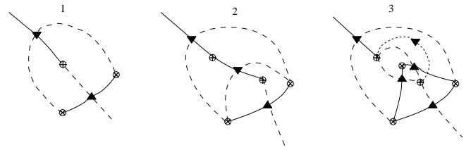
Fig. 5. A sequence of sketches of the important features in the topological footprints of the blinker group region during each of the three main phases. (a) is the initial intersecting state, (b) is the second stage which consists of two intersecting states, one inside the other, and (c) shows the final topology which includes a coronal null along with its associated spine. Positive sources are shown as \oplus , negative sources as \otimes , positive nulls as \blacktriangledown , and negative nulls as \blacktriangle . Spines (in the photosphere) are solid curves, separatrix traces are dashed, and the spine of the coronal null is dotted.
