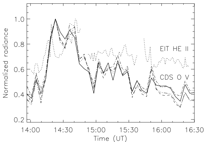
Fig. 2. Light curve of the blinker group (solid line), with the light curves for a sample of 3 individual blinkers (dashed and dotted line) as seen in CDS O v 629 \text{ \AA} . The EIT He II 304 \text{ \AA} light curve is shown for comparison.
